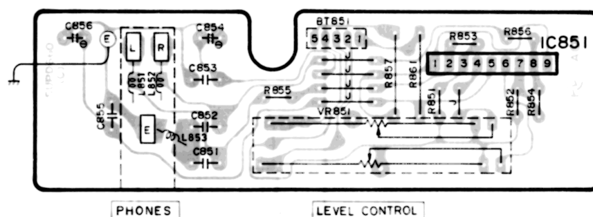
M HEADPHONE AMP P.C.B.
